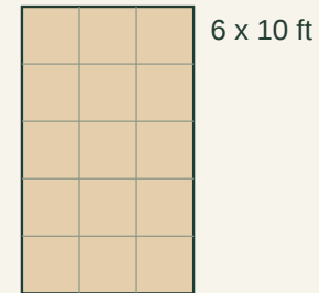
6-Chicken Coop + Covered Run
